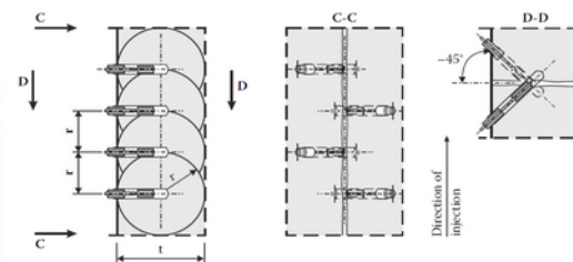
t: Crack depth r: Effective radius of a single packer and distance of each packer (max. 60 cm)
