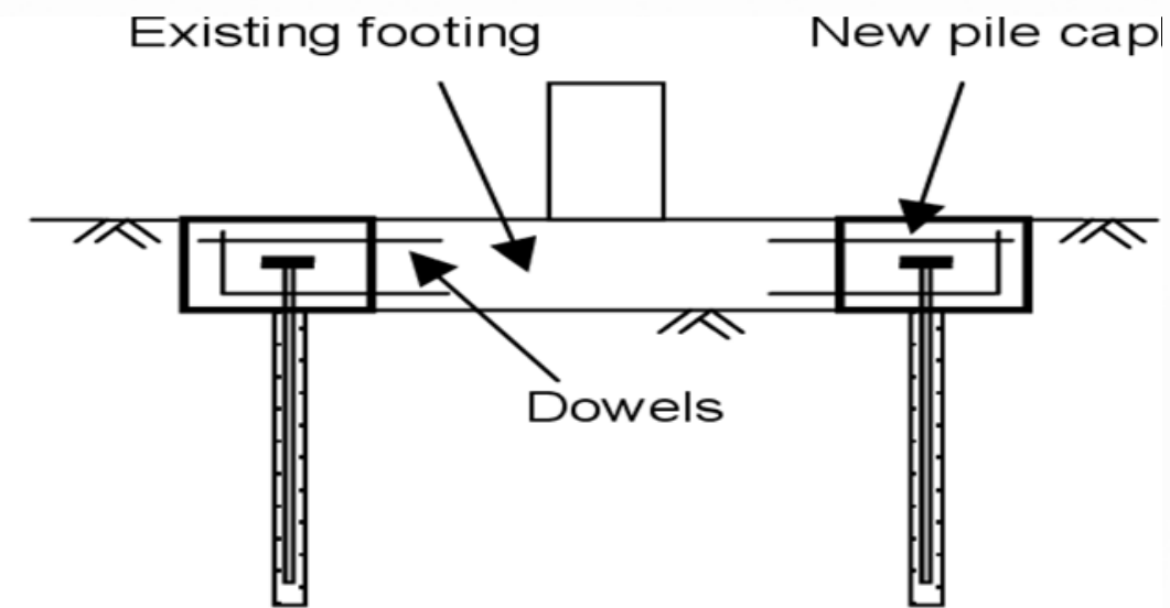
New pile cap attached to existing footing
