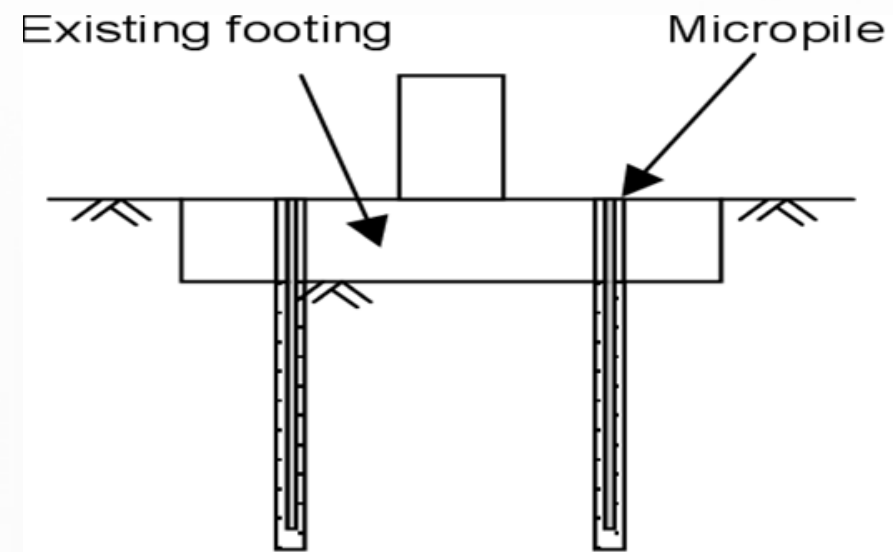
Micropiles through existing footing
